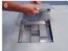
6 Remove the frame and trap by loosening the four corner
